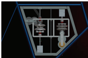
ProEngineer® CAD Model of Bicycle CVT (Continuously Variable Transmission): the model takes into account the materials used for each component.
