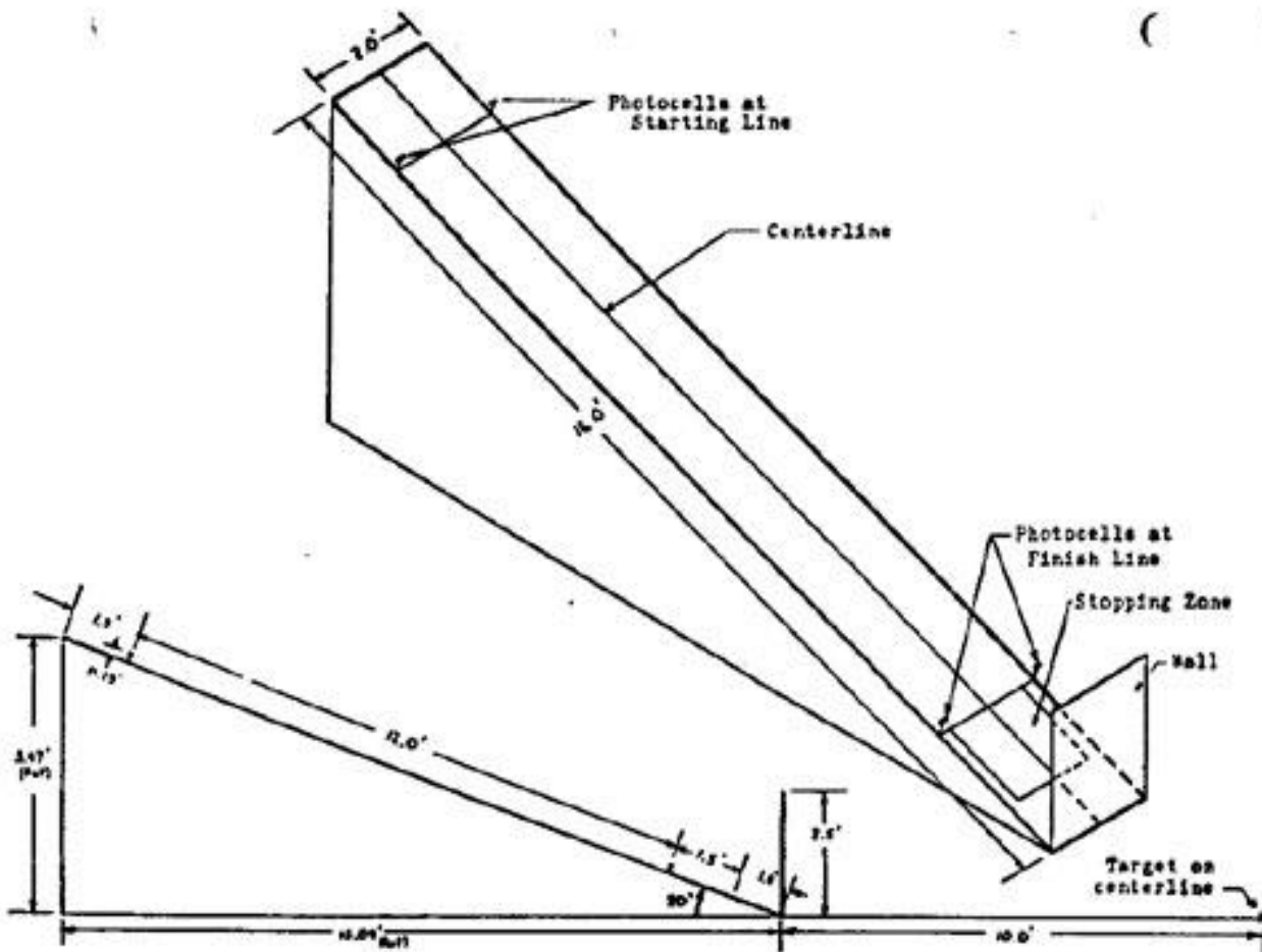
Figure 1 Detail of Ramp and Course for Tank Contest
