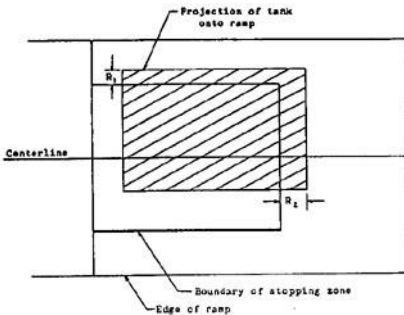
Figure 2 Example of Tank exceeding stopping zone boundaries in two directions. Since R_2 is greater than R_1 , the value of R_2 will be used in the score equation.
